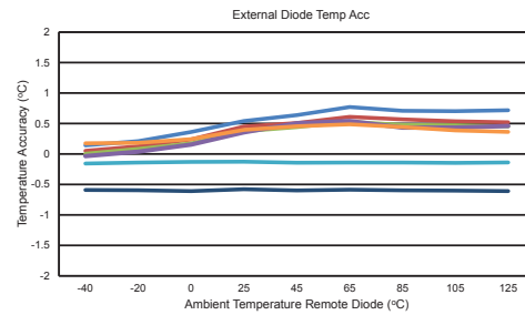
Figure 4-2. Temperature Accuracy vs. Remote Diode Temperature, V_{DD} = 1.8V
