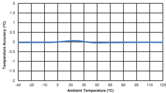
Figure 4-1. Internal Temperature Error vs. Ambient Temperature ( V_{DD} = 2.5V , T_D = +25^\circ C , 2N3904)
